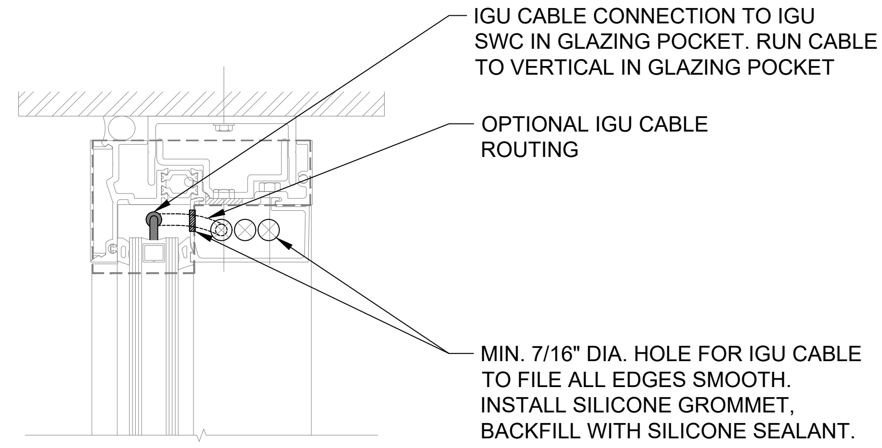
DETAIL 1 HEAD
