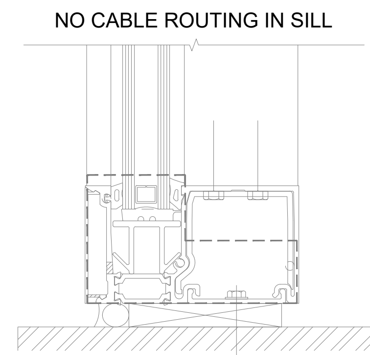
DETAIL 3 SILL
