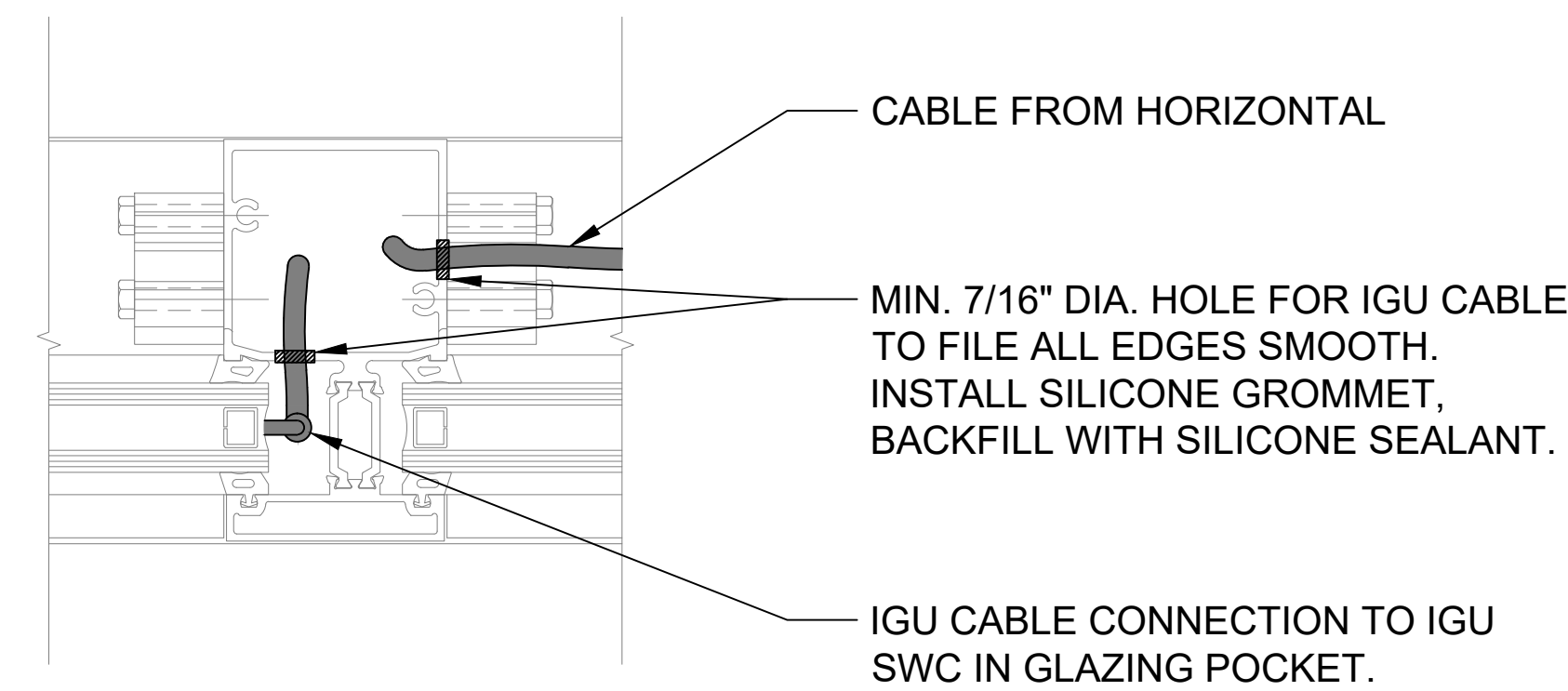
DETAIL 5 VERTICAL MULLION
